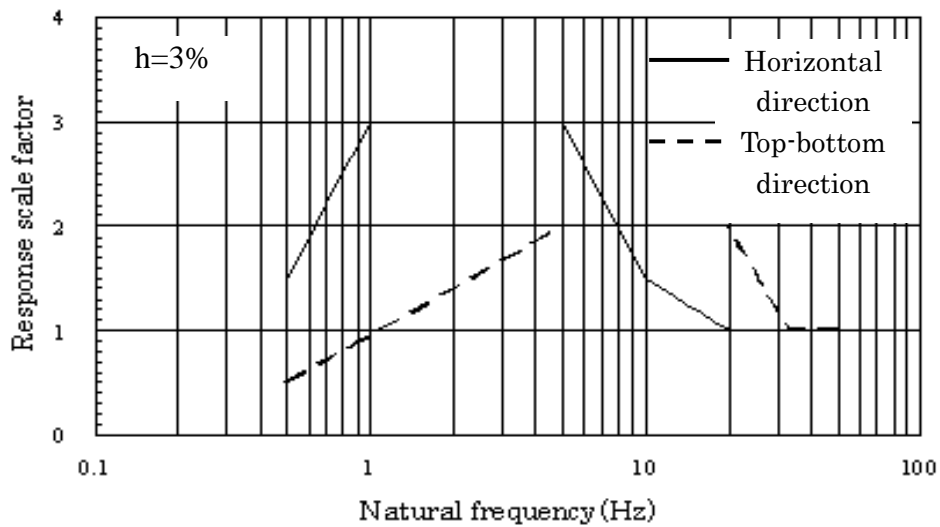
Figure 2 Acceleration Response Scale Factor of Excitation Waves ( h = 3\% )
