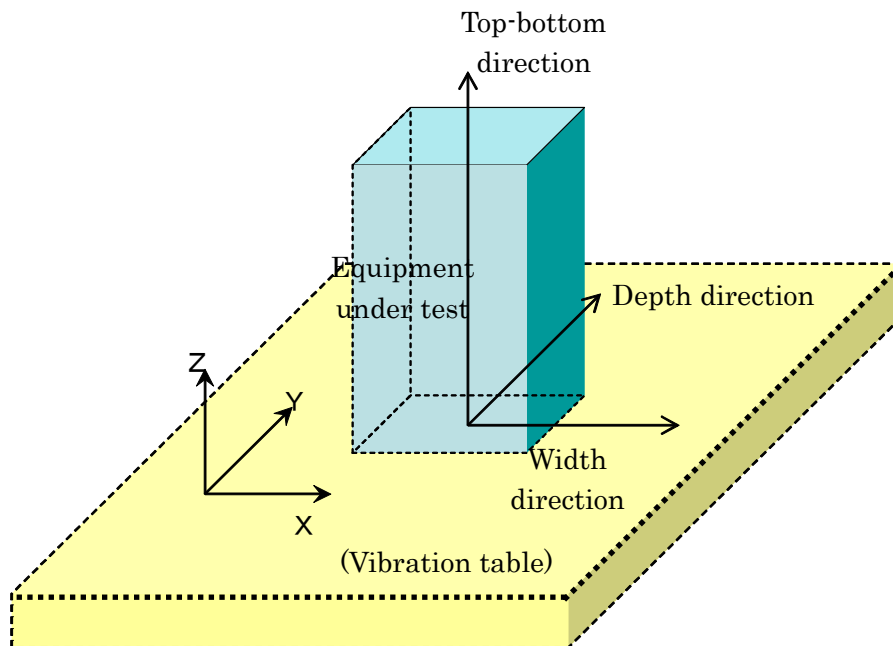
Figure 1 Simultaneous Excitation in 3 Directions (3-D Vibration Table)
