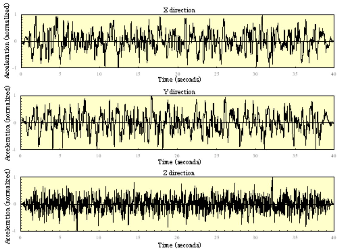
Figure 3 Time-based Excitation Waveforms (Maximum Acceleration normalized to 1)
